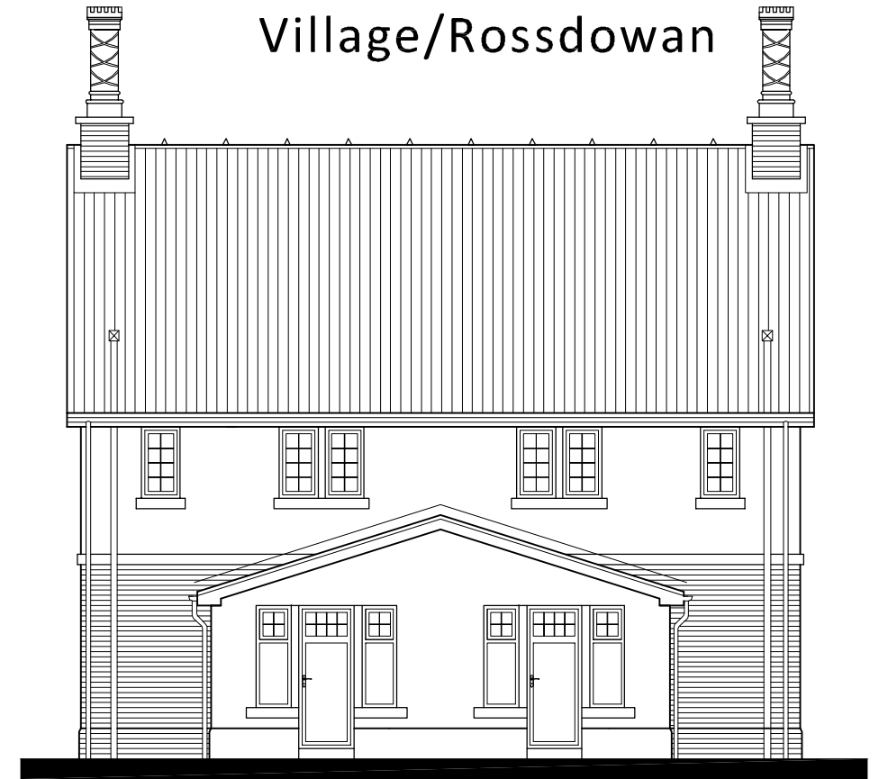
Rear Elevation
